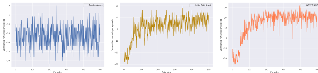
Figure 2: The performance of the three agents over 500 episodes in the non-stationary environment
