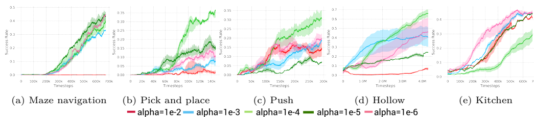
Figure 3: Learning rate \alpha ablation This figure compares the success rate performances for various values of primitive informed regularization weight \alpha hyper-parameter. If \alpha is too small, we lose the advantages of primitive informed regularization, leading to degrading performance. In contrast, if \alpha is too large, it may lead to degenerate solutions. Thus, these success rate performance plots demonstrate that proper primitive subgoal regularization is crucial for appropriate subgoal prediction, and improving overall performance.
