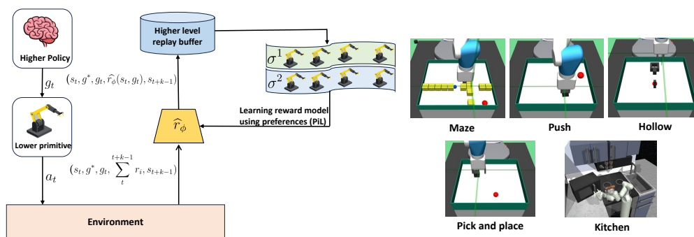
Figure 1: PIPER Overview This figure shows the overview of PIPER (left). The higher level policy predicts subgoals g_t for the lower primitive, which executes actions a_t on the environment. We propose to learn a preference-based reward model \hat{r}_\phi using our PiL feedback on higher level trajectories sampled from higher level replay buffer, and subsequently use \hat{r}_\phi to relabel the replay buffer transitions, thereby mitigating non-stationarity in HRL. On the right, we depict the training environments: (i) maze navigation environment, (ii) pick and place environment, (iii) push environment, (iv) hollow environment, and (v) franka kitchen environment.
