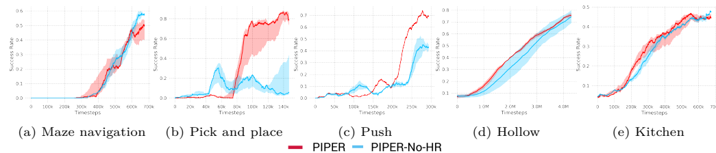
Figure 4: Hindsight Relabeling ablation This figure compares the performance of our PIPER approach with PIPER-No-HR ablation, which is effectively PIPER without hindsight relabeling ( Andrychowicz et al., 2017 ) (as explained in Section 4.3). The plots showcase that although hindsight relabeling demonstrates minor performance improvement in sparse maze and kitchen tasks, it provides significant training speedup in sparse pick and place and push environments.
